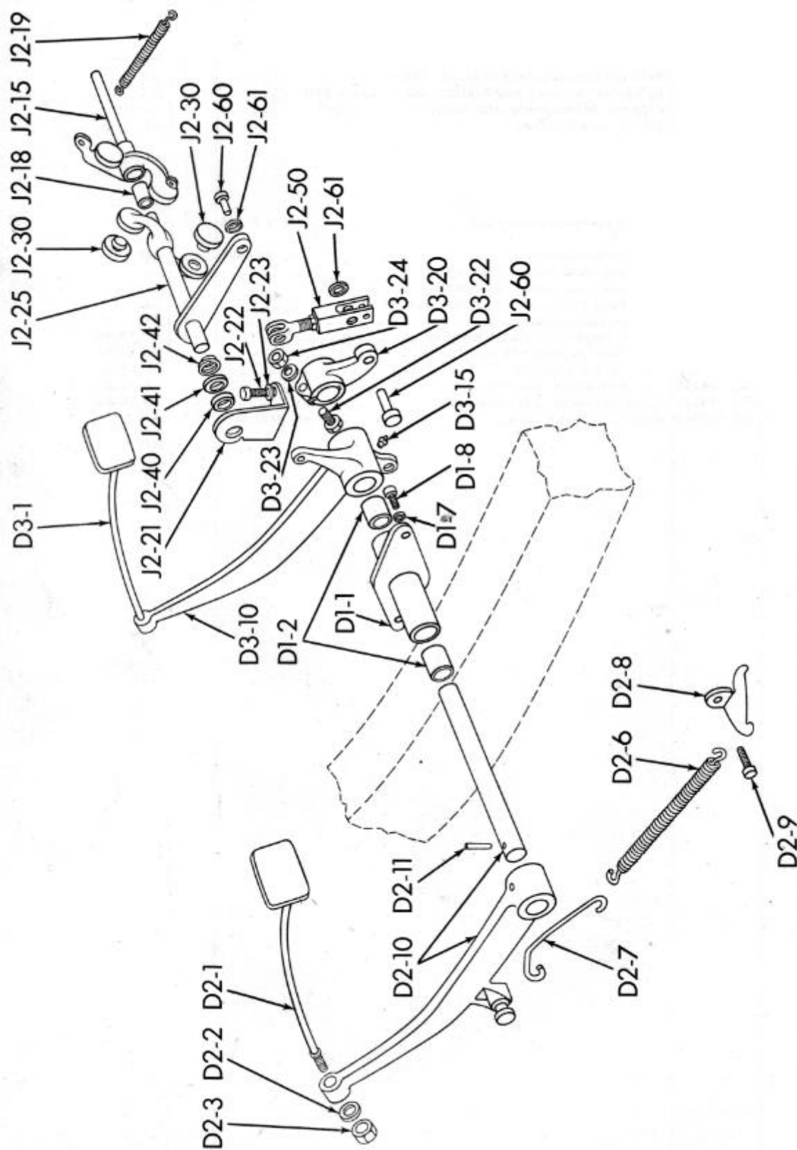
Clutch Control
