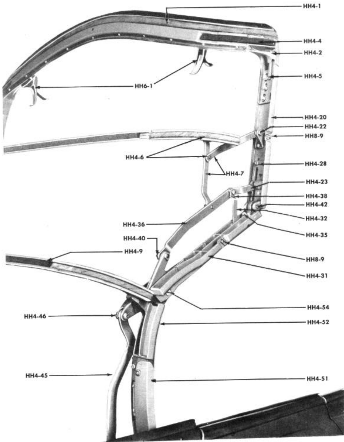
Folding Top - Convertible
