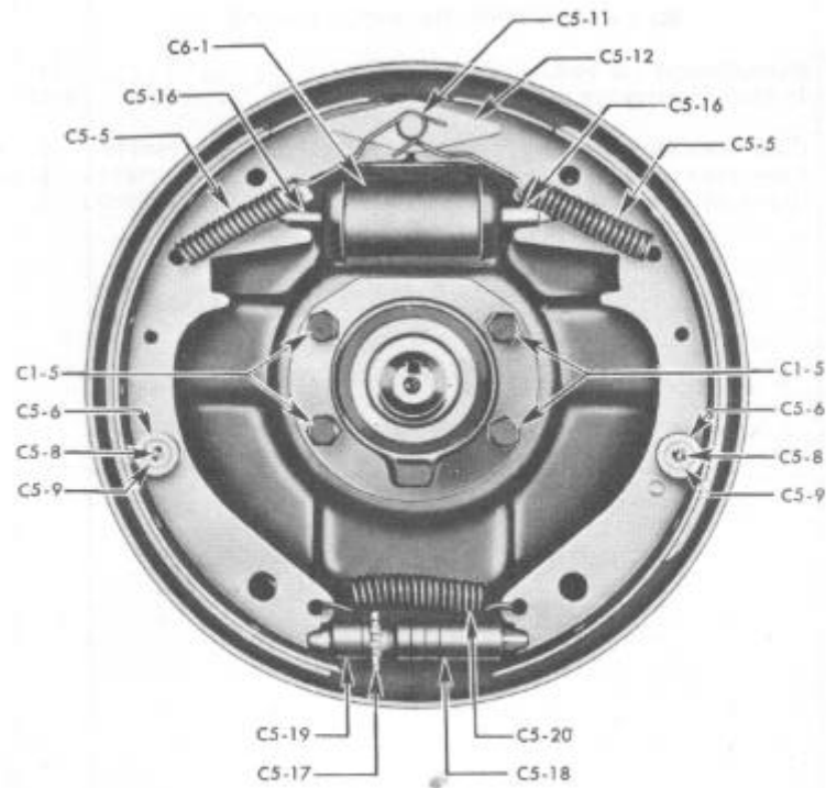
Front Brake
