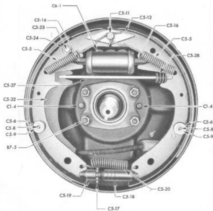
Rear Brake
