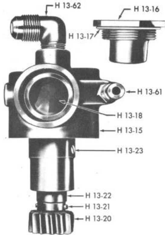
Oil Pump - Eight Cylinder Engine
