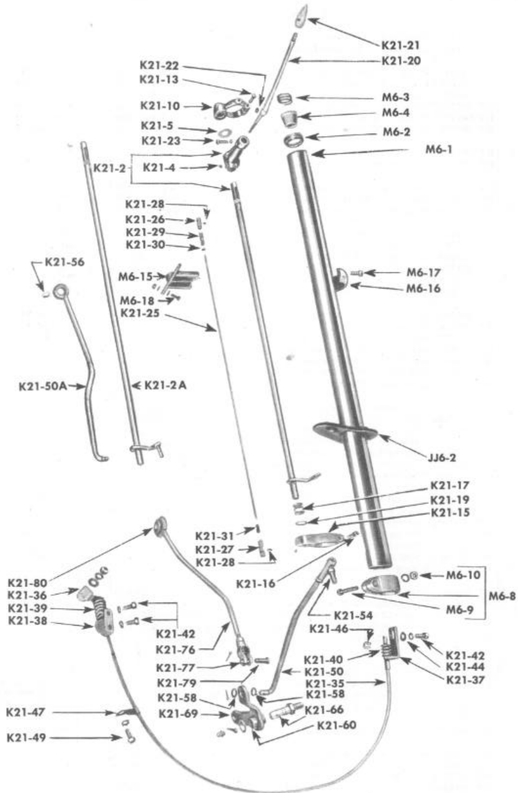
Handy Shift - First Series
