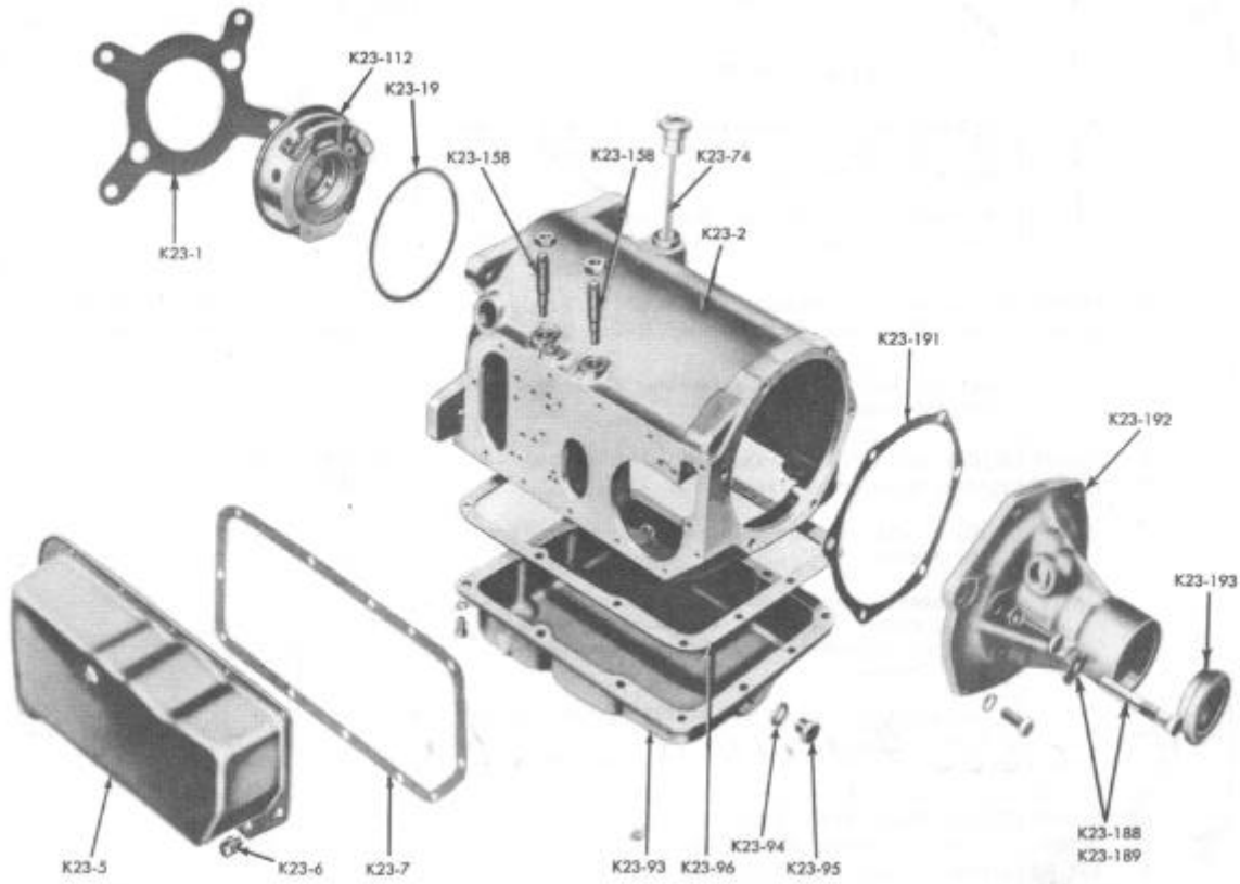
CASE, COVERS AND REAR BEARING CONTAINER — HYDRA-MATIC TRANSMISSION
