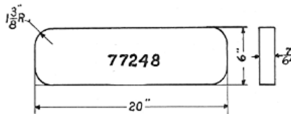
Rear Glass No. 77248
