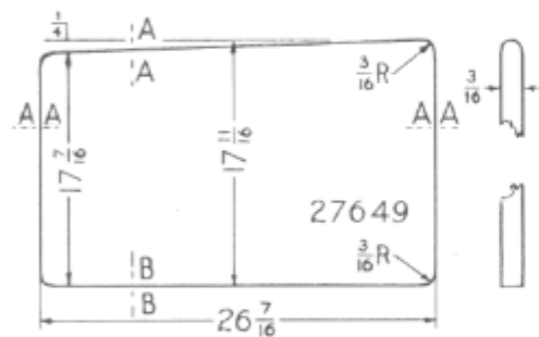
Front Door Glass No. 27649
