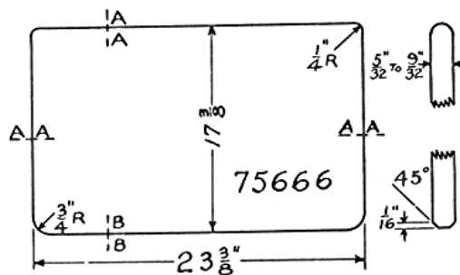
Front and Rear Door Glass No. 75666
