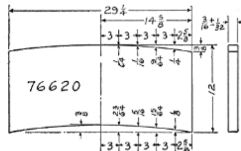
Rear Glass No. 76620
