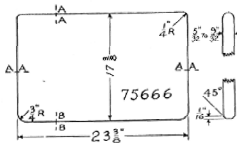
Door Glass No. 75666
