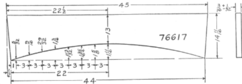
Windshield Glass No. 76617
