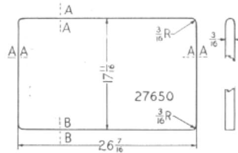
Rear Door Glass No. 27650
