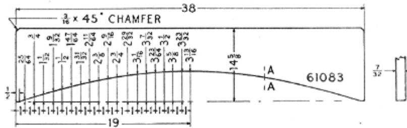
Windshield Glass No. 61083
