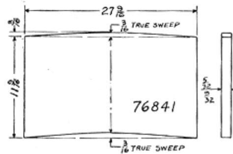
Rear Glass No. 76841
