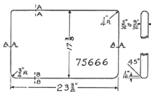
Door Glass No. 75666
