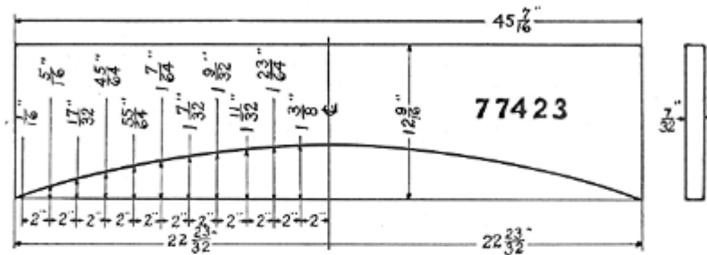
Windshield Glass No. 77423
