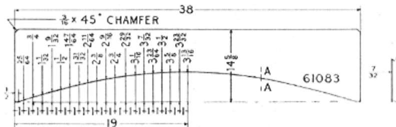
Windshield Glass No. 61083
