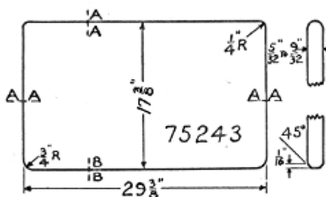
Door Glass Right and Left No. 75243
