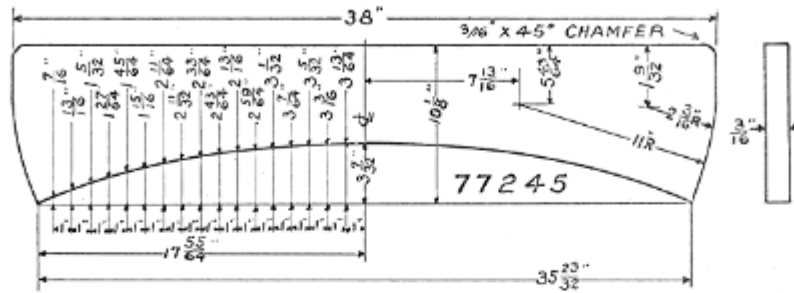
Windshield Glass No. 77245
