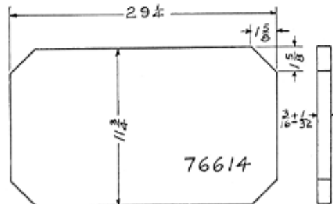
Rear Glass No. 76614
