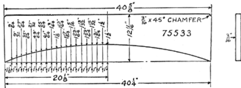
Windshield Glass No. 75533
