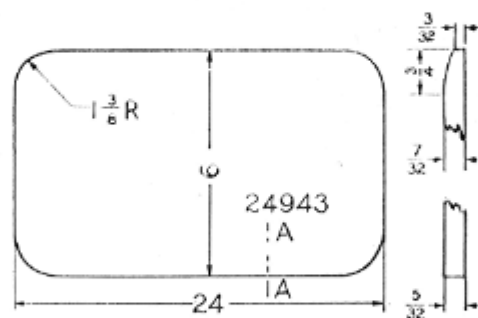
Rear Glass No. 24943
