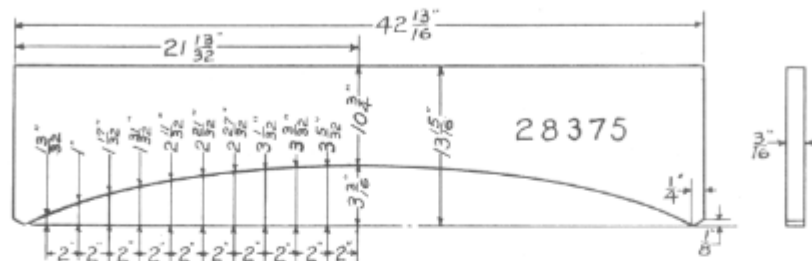
Windshield Glass No. 28375
