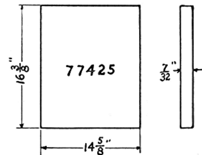
Quarter Glass No. 77425
