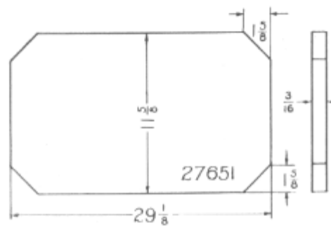
Rear Glass No. 27651
