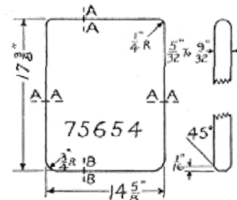
Quarter Glass No. 75654
