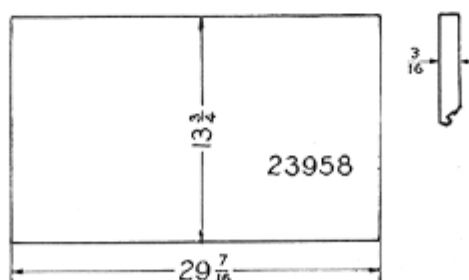
Rear Glass No. 23958
