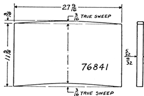
Rear Glass No. 76841
