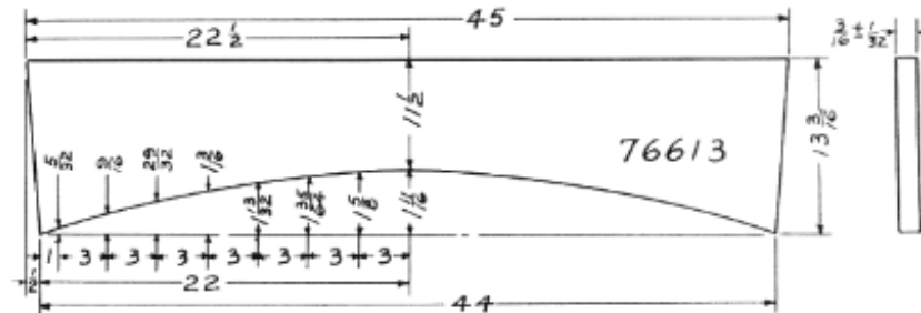
Windshield Glass No. 76613
