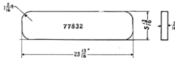
Rear Glass No. 77832
