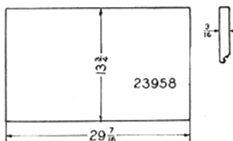
Rear Window Glass No. 23958
