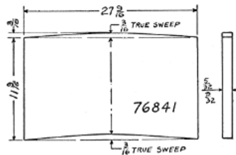
Rear Glass No. 76841
