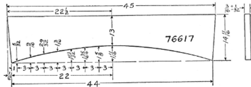
Windshield Glass No. 76617
