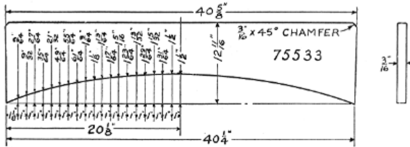
Windshield Glass No. 75533
