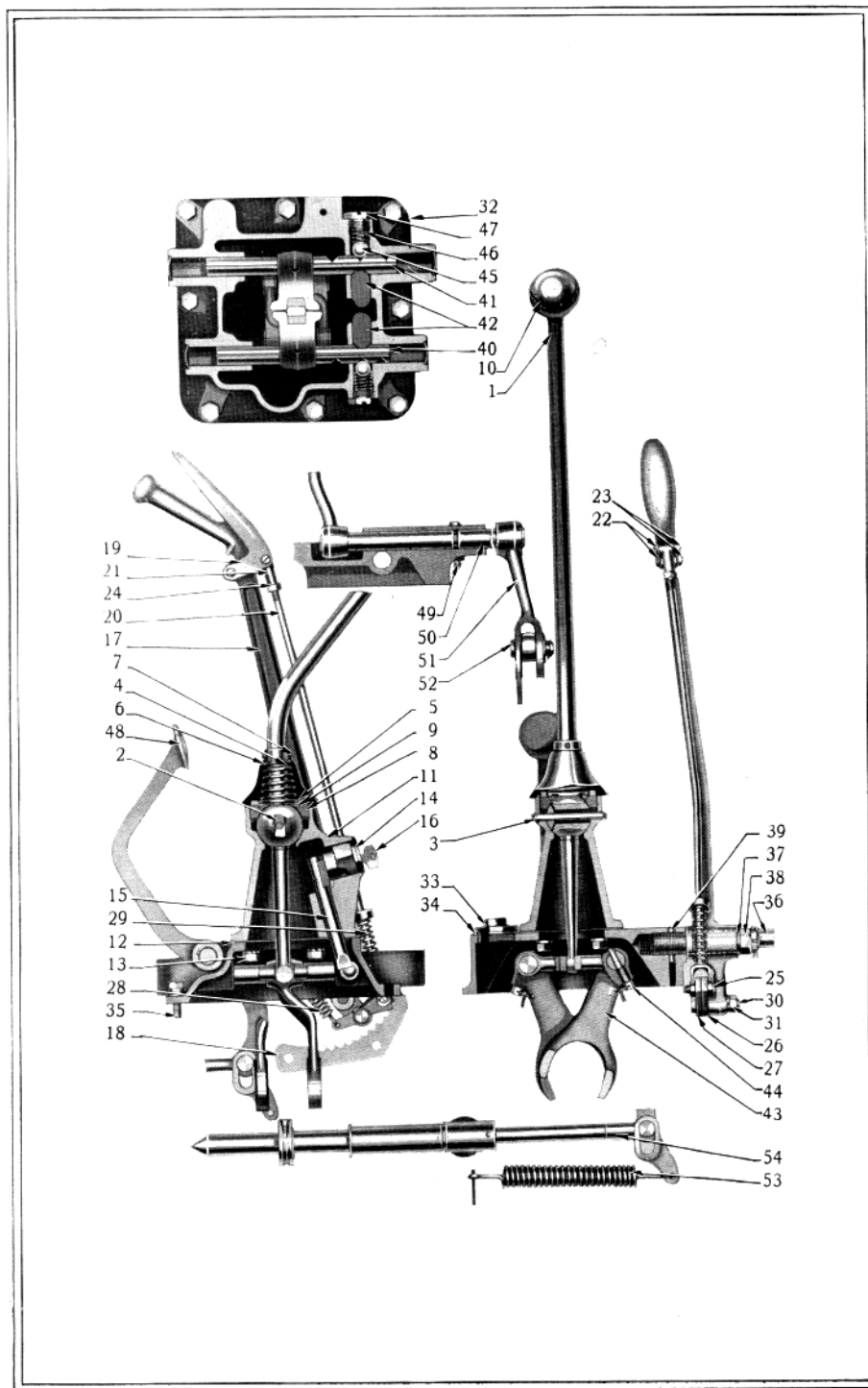
Hand Control Assembly
