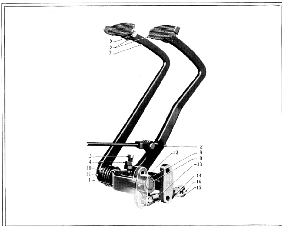
Pedal Control Assembly
