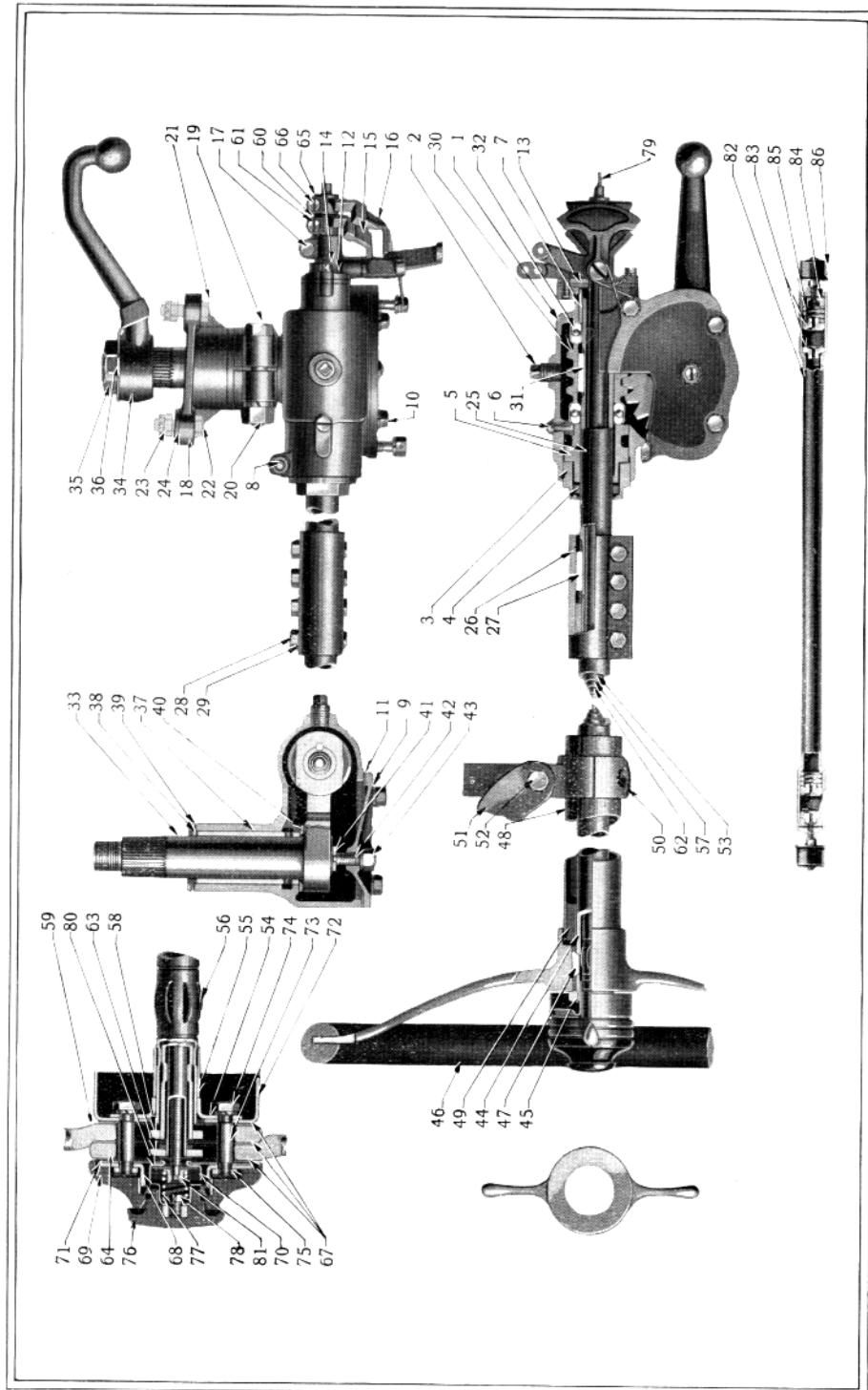
Steering Gear Assembly
