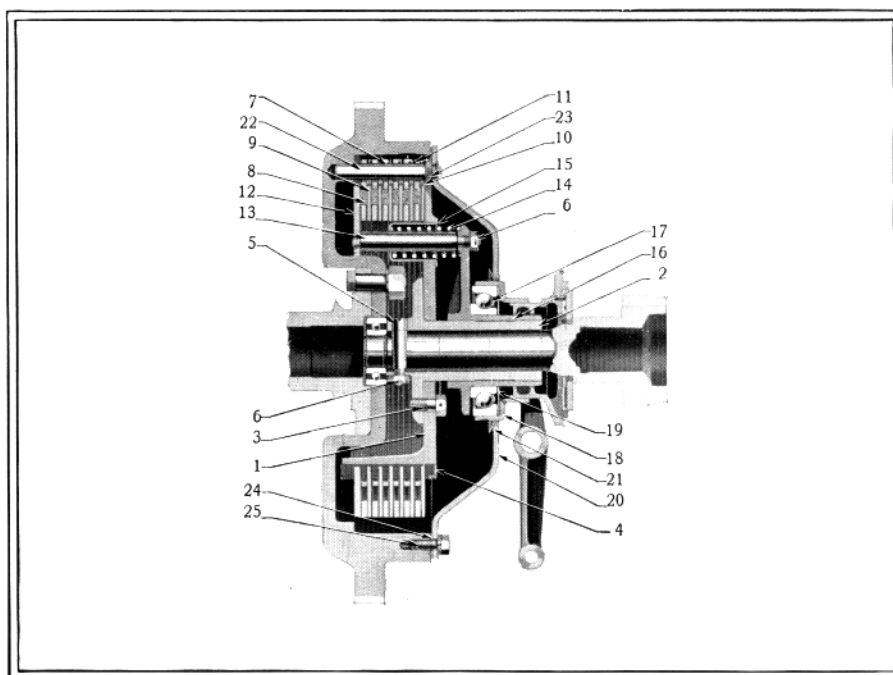
Clutch Assembly
