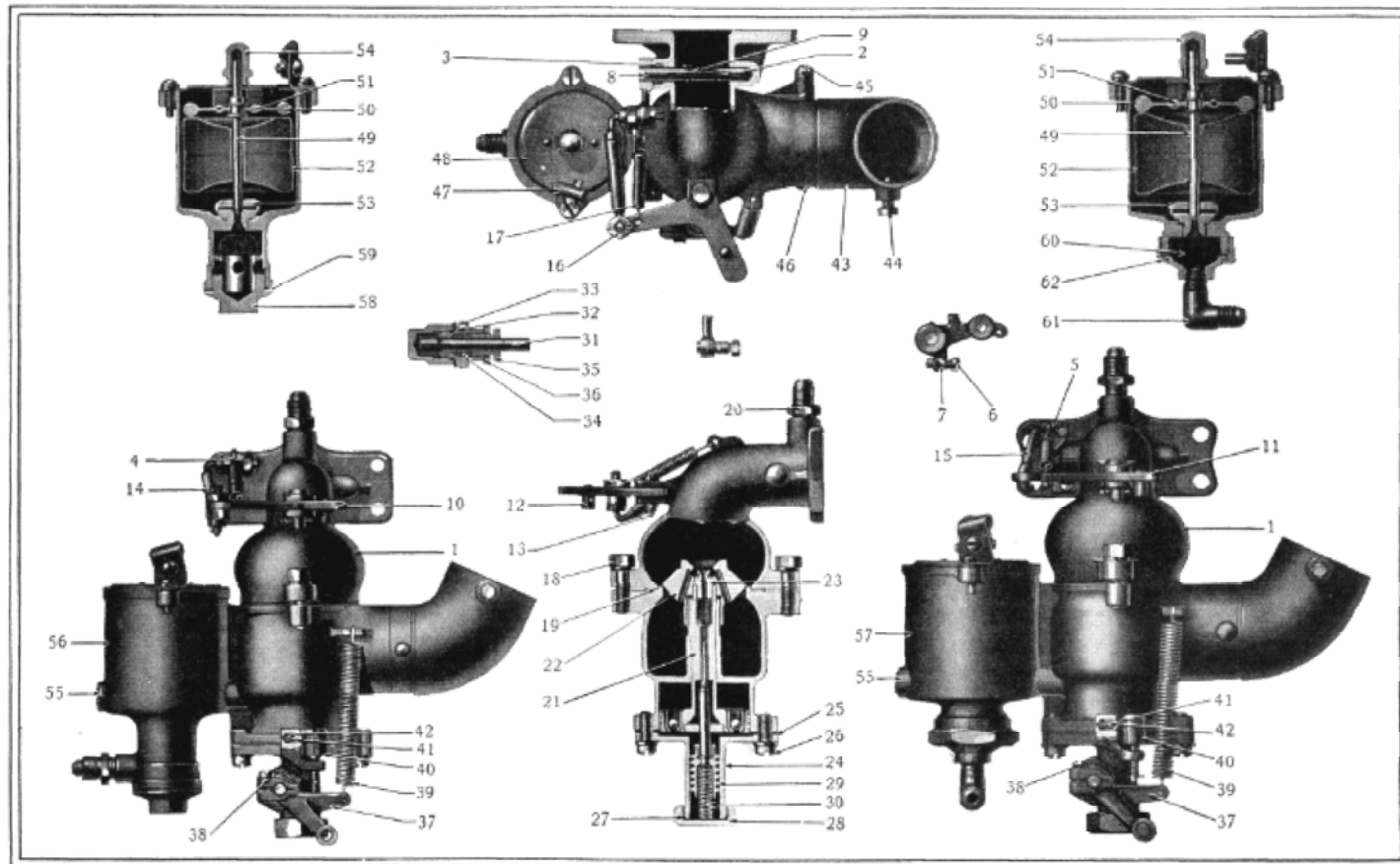
CARBURETOR ASSEMBLY
