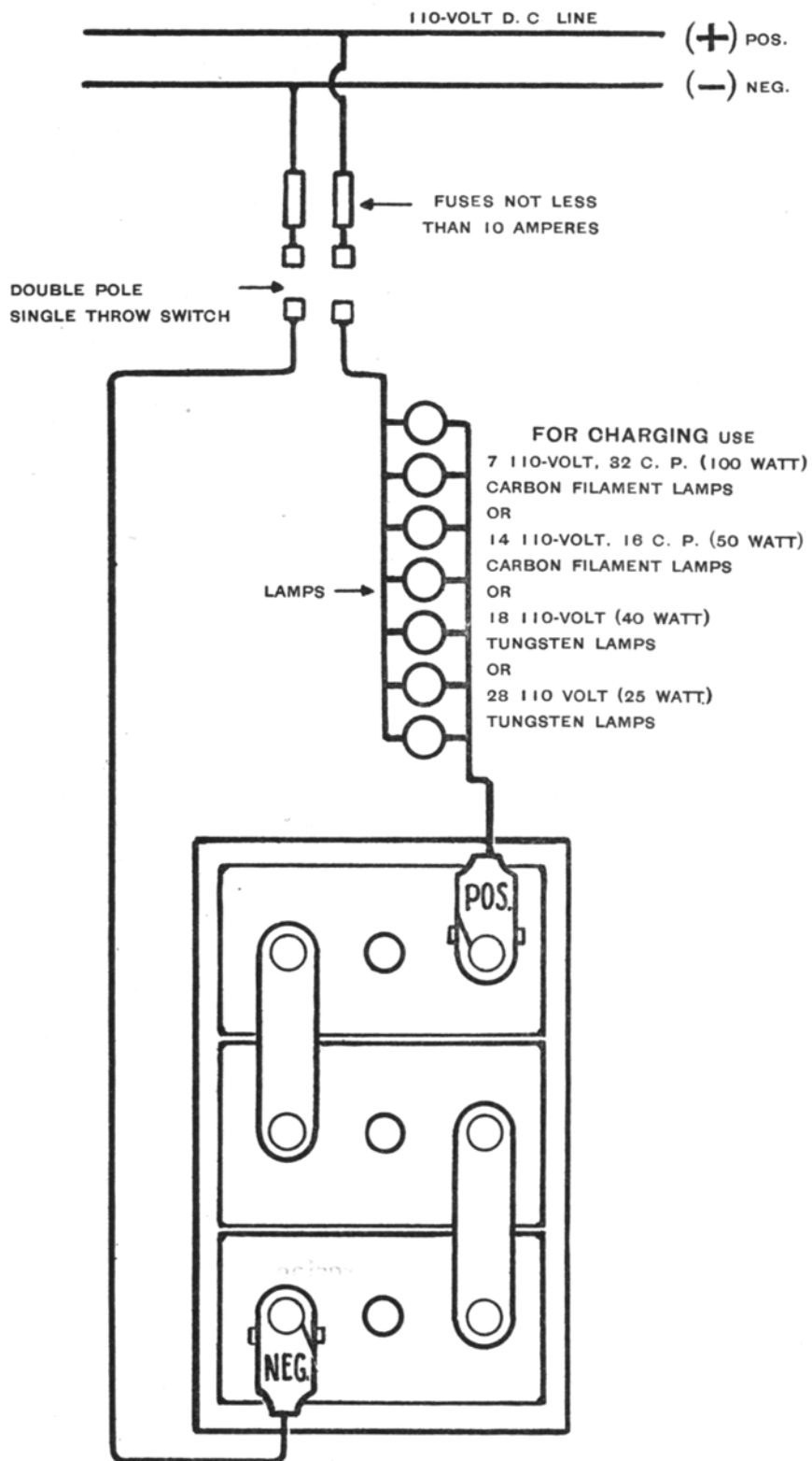
Charging Circuit Diagram
