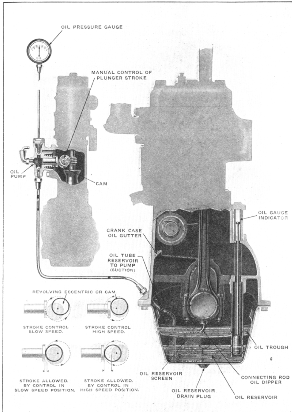
Details of Oiling System
