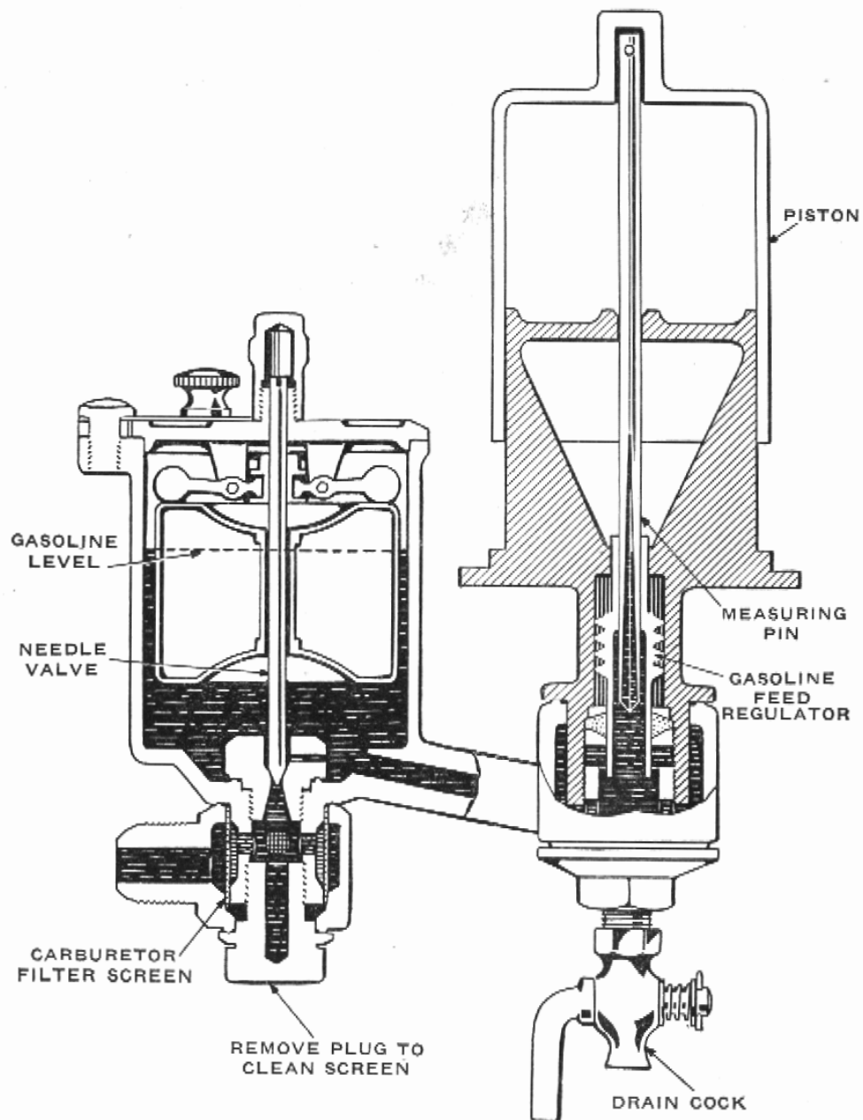
Carburetor Gasoline Level
