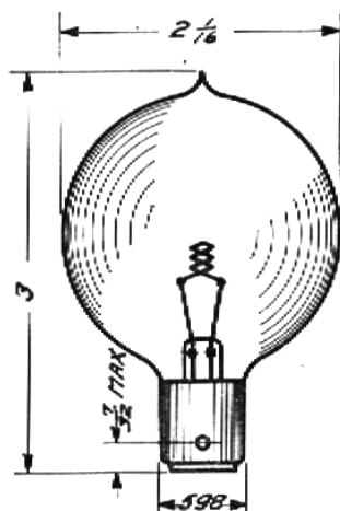
Head Lamp Bulb
