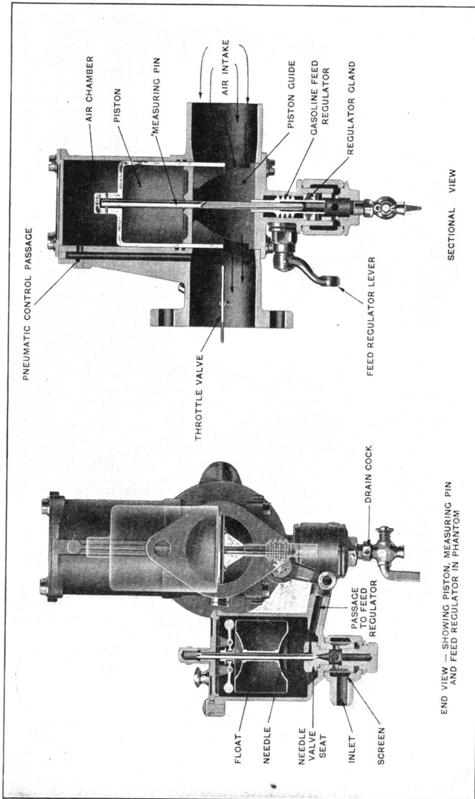
The Hudson Carburetor
