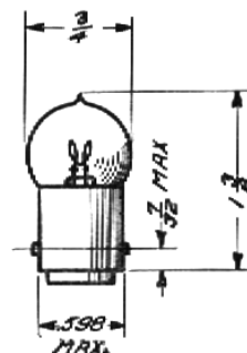
Tail and Dash Lamp Bulb
