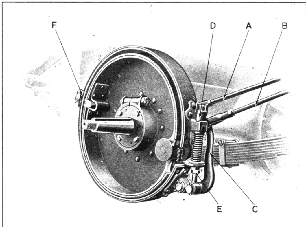
Brake Adjustment
