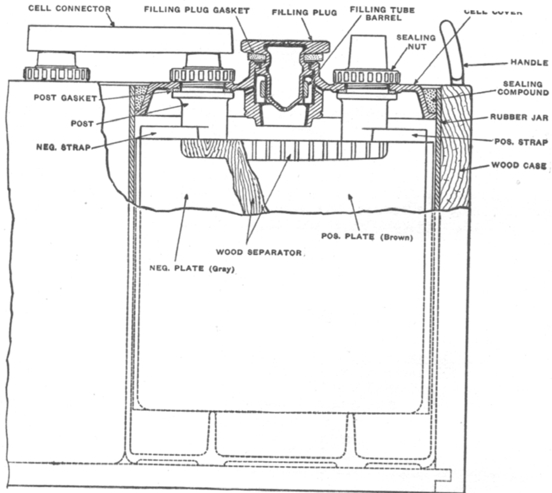
Storage Battery
