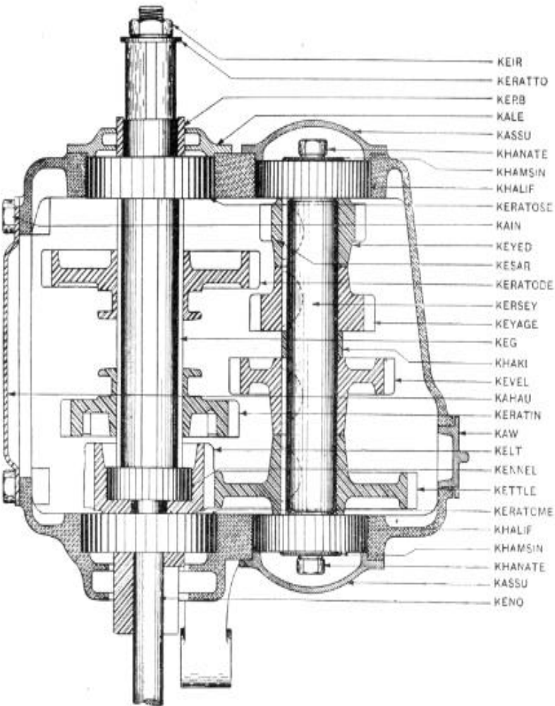
TRANSMISSION SHAFT SECTION
