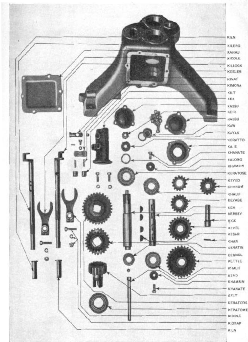
TRANSMISSION ASSEMBLY
